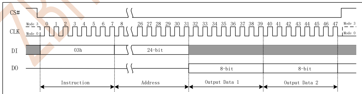
Figure 7.9 Read Data Instruction
