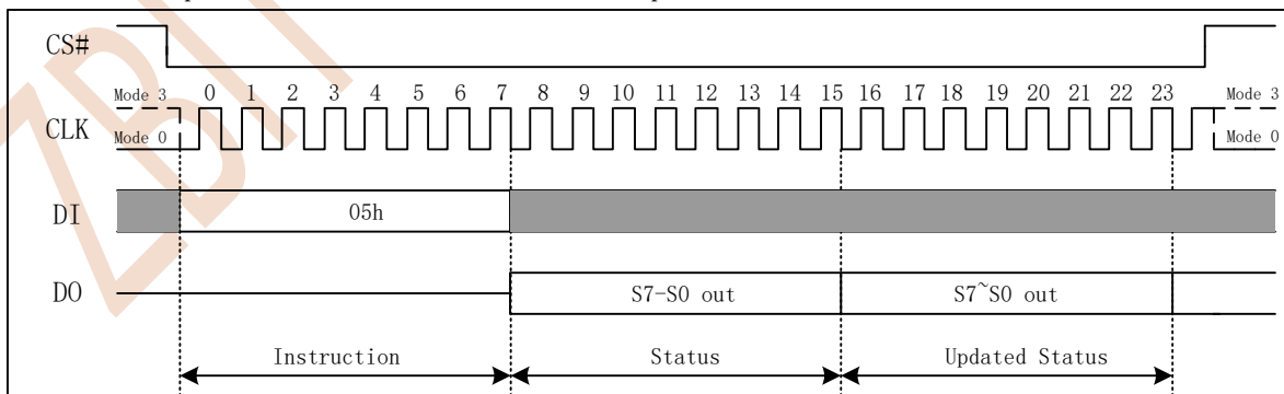
Figure 7.1 Read Status Register Instruction
