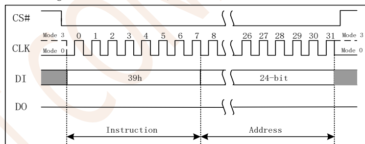
Figure 7.32a Individual Block/Sector Unlock Instruction(SPI Mode)
