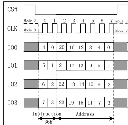
Figure 7.31b Individual Block/Sector Lock Instruction(QPI Mode)
