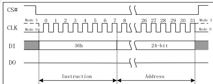
Figure 7.31a Individual Block/Sector Lock Instruction (SPI Mode)
