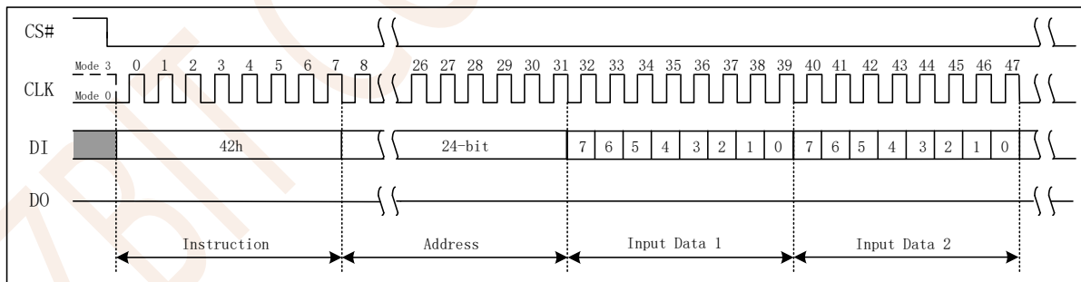
Figure 7.29 Program Security Registers Instruction
