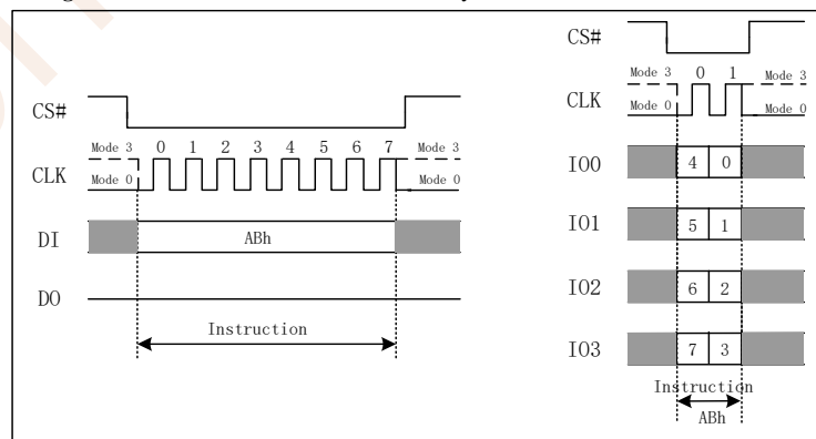
Figure 7.23 Release Power-down Instruction(SPI and QPI Mode)
