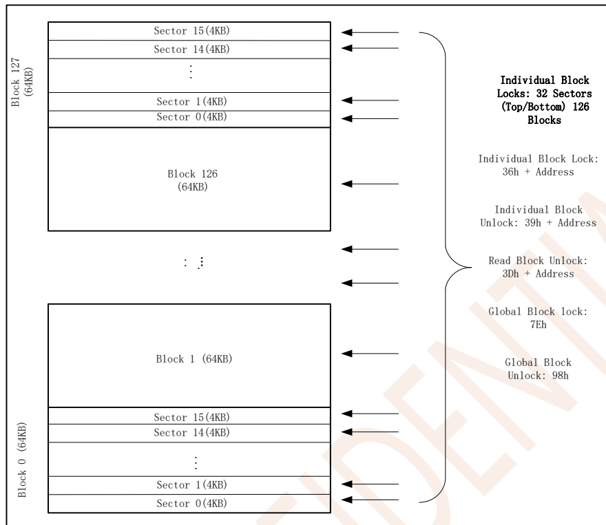
Figure 6.2 Individual Block/Sector Locks
