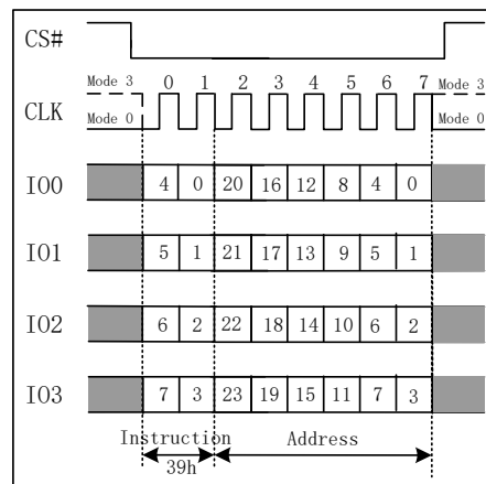
Figure 7.32b Individual Block/Sector Unlock Instruction(QPI Mode)
