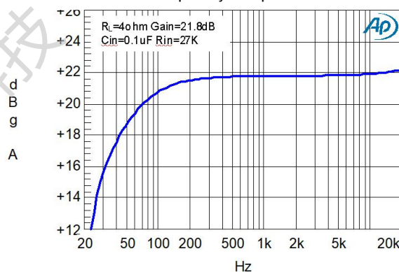
Frequency Response
