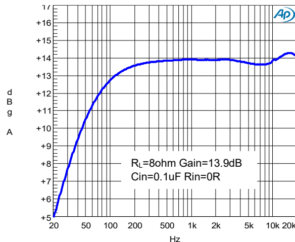
Frequency Response
