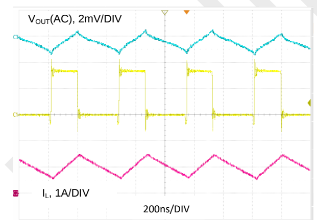
图 14. V_{OUT} = 1.2\text{V} , I_o = 1\text{A} , FPWM
