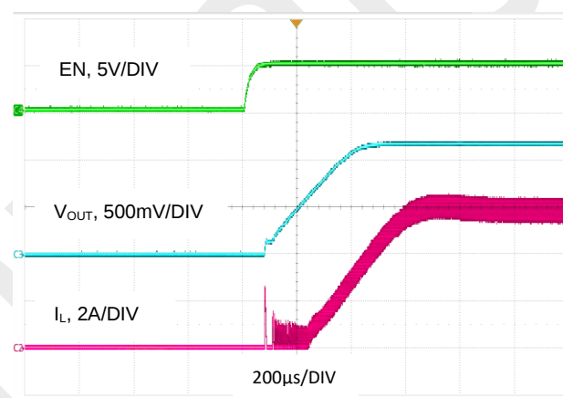
图 13. 启动波形, V_{OUT} = 1.2\text{V} , I_o = 6\text{A}
