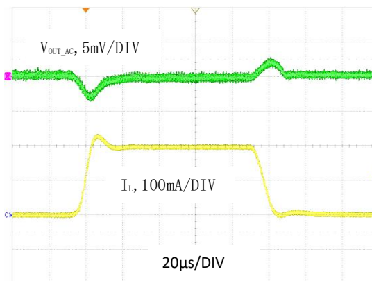
图 22. 负载瞬态响应, V_{IN}=4V , V_{OUT}=3.3V , I_{OUT}=1mA to 200mA
