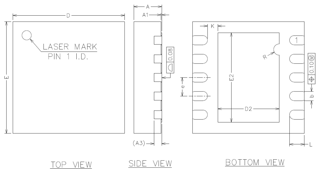
COMMON DIMENSIONS (UNITS OF MEASURE=MILLIMETER)
