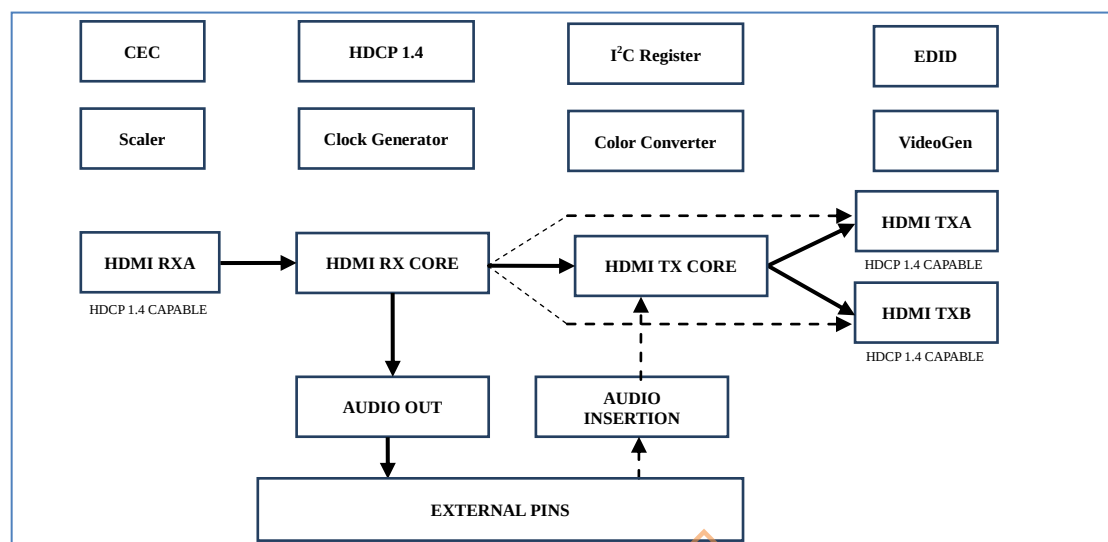
Figure 1. GSV1001 audio extraction diagram
