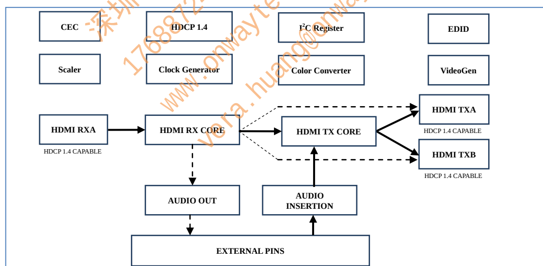
Figure 2. GSV1001 audio insertion diagram
