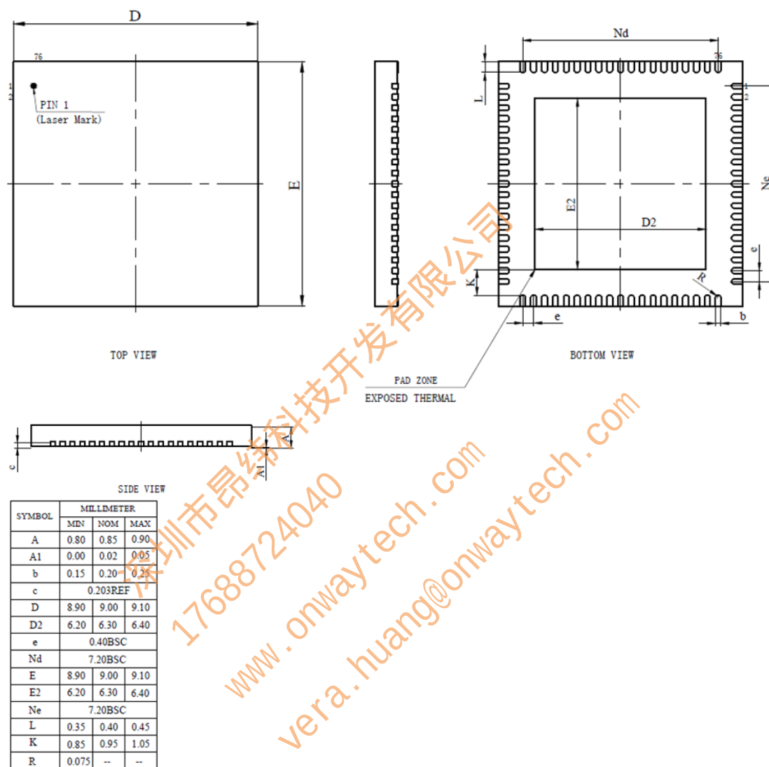
Figure 10. GSV1001 package dimensions
