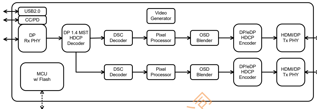
Figure 7. DP MST (compressed streams) to DP/eDP Conversion
