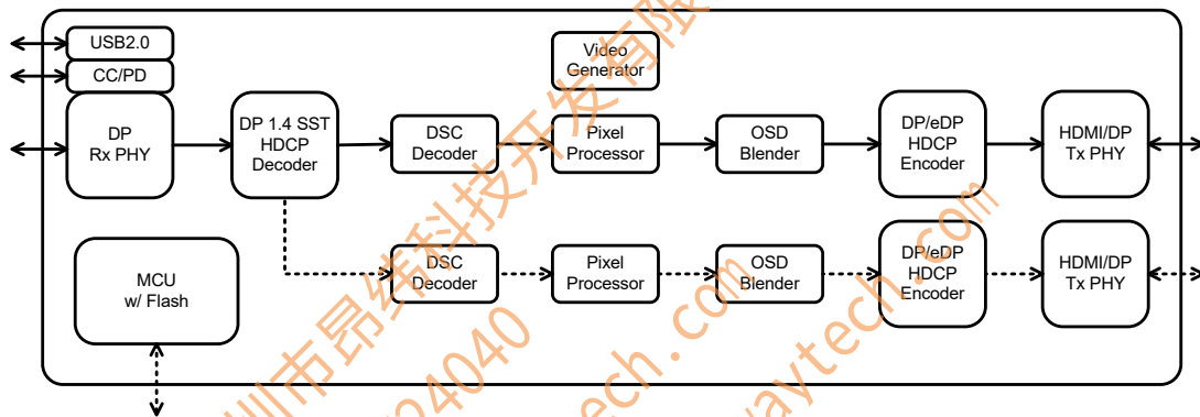
Figure 5. DP SST to DP/eDP Conversion
