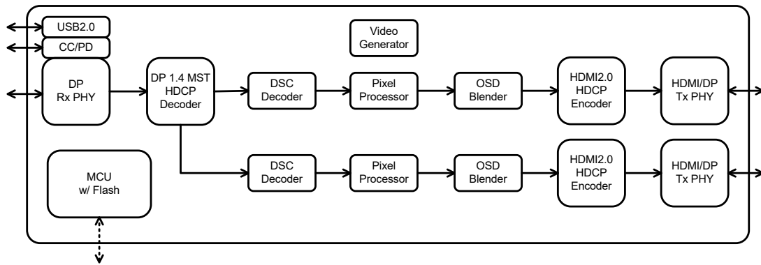
Figure 4. DP MST (compressed streams) to HDMI Conversion
