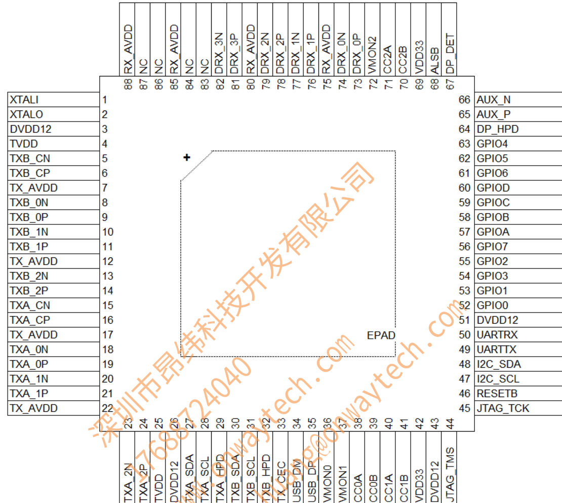
Figure 8. GSV2221G QFN88 Pin Diagram
