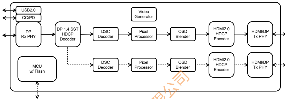
Figure 2. DP SST to HDMI Conversion
