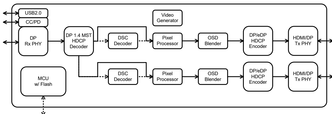
Figure 6. DP MST (uncompressed streams) to DP/eDP Conversion
